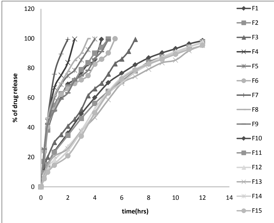
Fig 2 .Dissolution Profiles of Zidovudine SR Tablets
