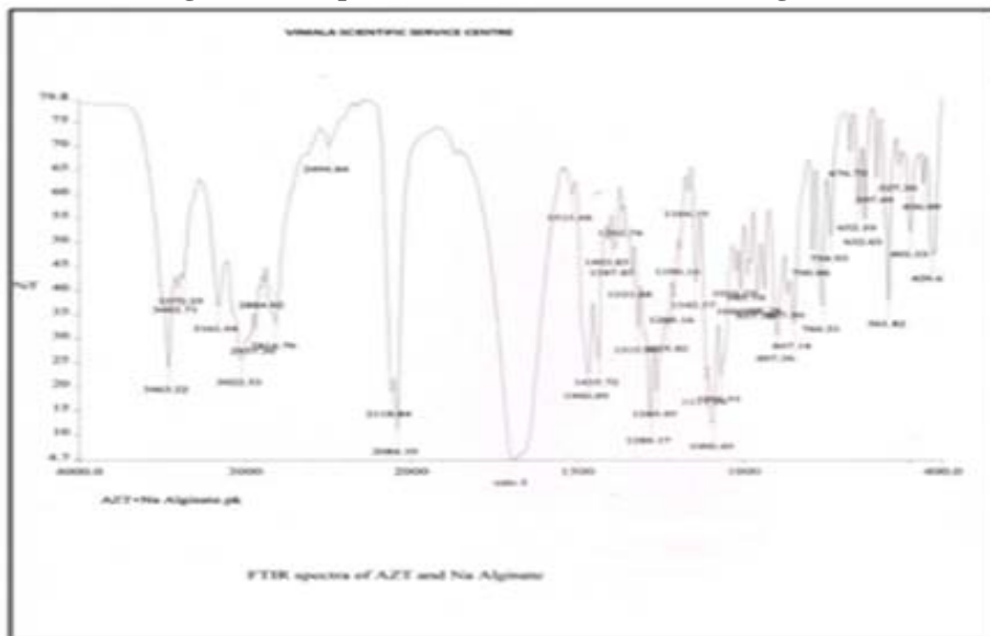
Fig.1.2. FTIR spectra of zidovudine and sodium alginate
